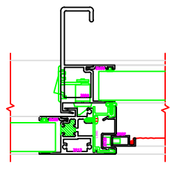
601 MEETING RAIL SERIES: 3500
