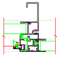
602 MEETING RAIL SERIES: 3500
